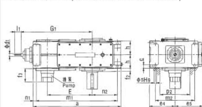
V4SV, V4HV, V4DV ( 强制润滑 With forced lubrication )
