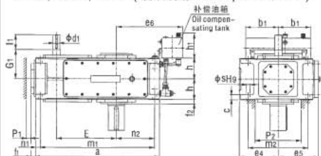
P2SV, P2HV, P2DV ( 浸油润滑 With dip lubrication )
