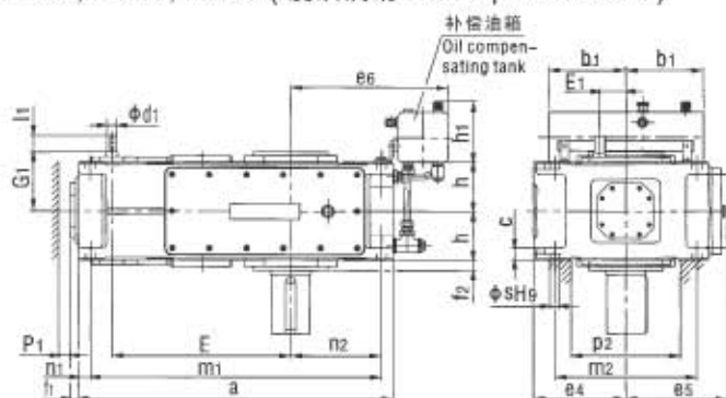
P4SV, P4HV, P4DV ( 浸油润滑 With dip lubrication )
