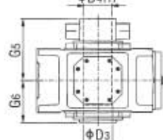
P2DV 带胀紧盘的空心轴 Hollow shaft for shrink disk
