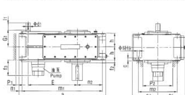
P3SV, P3HV, P3DV ( 强制润滑 With forced lubrication )
