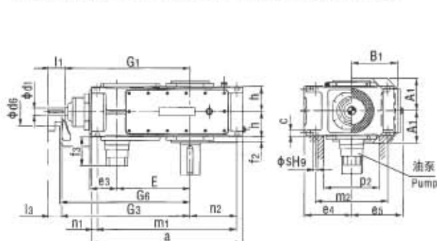
V3DV 带胀紧盘的空心轴 Hollow shaft for shrink disk
