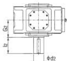
P2SV 实心轴 Solid shaft
