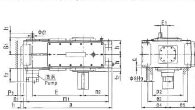
P4SV, P4HV, P4DV ( 强制润滑 With forced lubrication )
