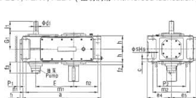
P2SV, P2HV, P2DV ( 强制润滑 With forced lubrication )
