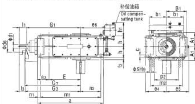
V3SV, V3HV, V3DV ( 浸油润滑 With dip lubrication )
