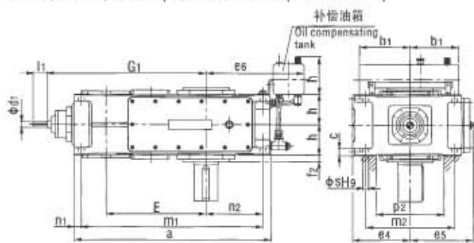
V4SV, V4HV, V4DV ( 浸油润滑 With dip lubrication )
