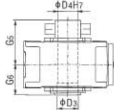
P3DV 带胀紧盘的空心轴 Hollow shaft for shrink disk
