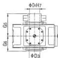
V4DV 帶脹緊盤的空心軸 Hollow shaft for shrink disk
