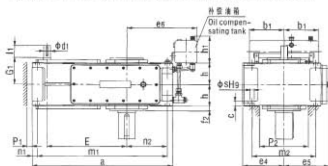
P3SV, P3HV, P3DV ( 浸油润滑 With dip lubrication )
